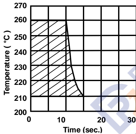
<Allowable Reflow Soldering Temp. and Time>
